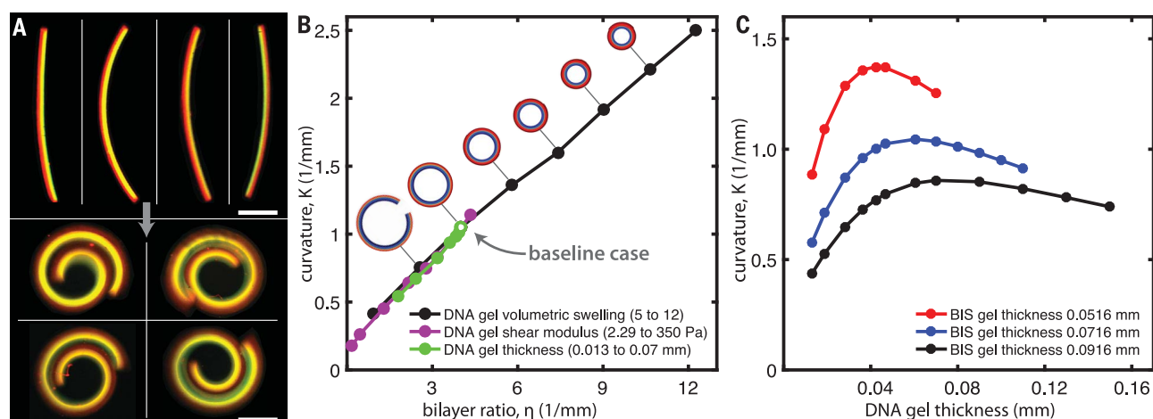
Fig. 3. Shape-change mechanics. (A) Fluorescence micrographs of photopatterned hydrogel beams (side views) with a 60- \mu m-thick BIS-cross-linked polyacrylamide layer (green) and a 60- \mu m-thick DNA-cross-linked hydrogel (red), before (top) and after (bottom) sequence-driven curving. Scale bars, 1 mm. (B) Computational finite element parameter study of bilayer curvature. The baseline case (white circle) corresponds to the experimentally measured
