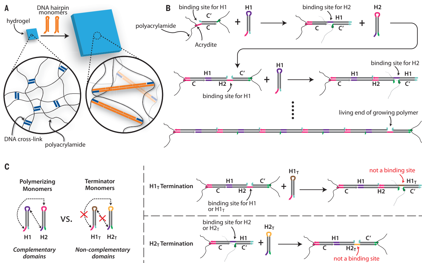
Fig. 1. DNA-directed expansion of DNA-cross-linked polyacrylamide gels. (A) DNA-cross-linked polyacrylamide hydrogels (8). Hairpins can insert into cross-links, inducing hydrogel expansion. (B) Schematic of cross-link C-C' extension by hairpins H1 and H2. Colors indicate domain
